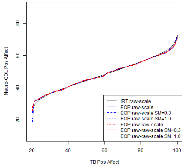
Figure 5.26.10: Equipercentile Linking Functions
