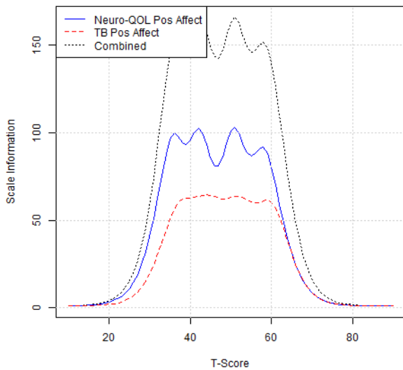
Figure 5.26.7: Comparison of Scale Information Functions
