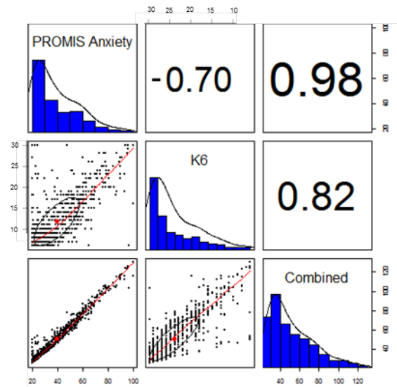
Figure 5.13.4: Scatter Plot Matrix of Raw Summed Scores
