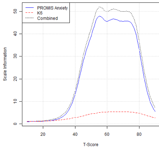
Figure 5.13.7: Comparison of Scale Information Functions
