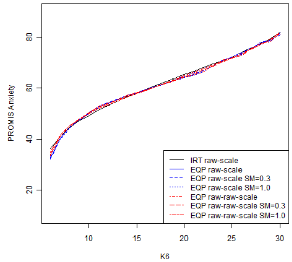
Figure 5.13.10: Equipercentile Linking Functions
