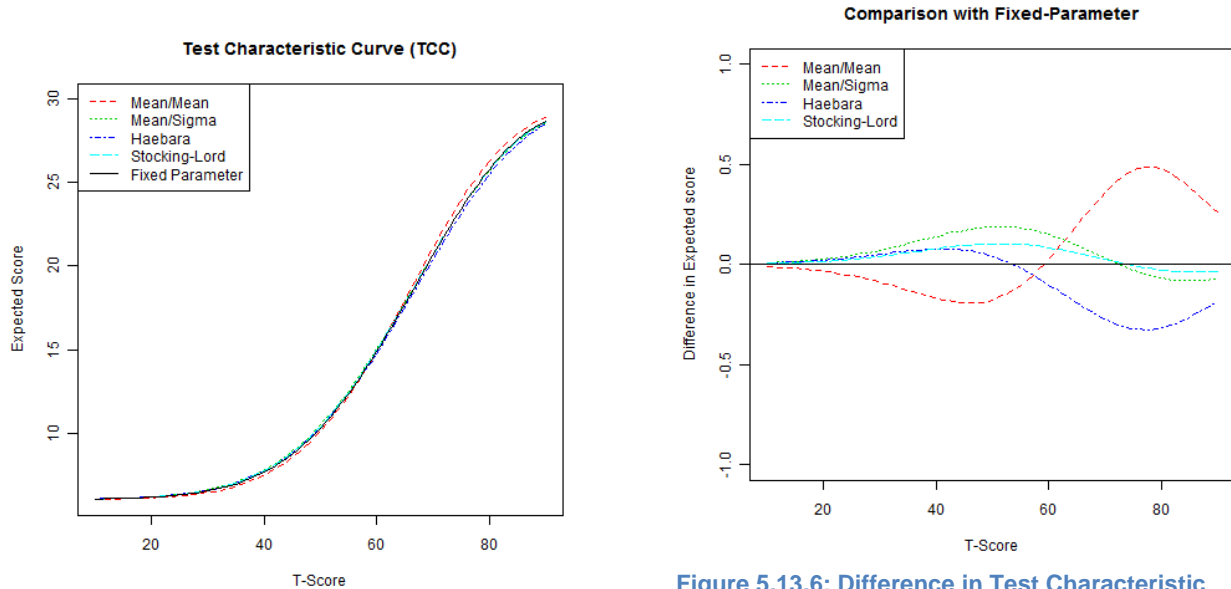
Figure 5.13.5: Test Characteristic Curves (TCC) from Different Linking Methods
