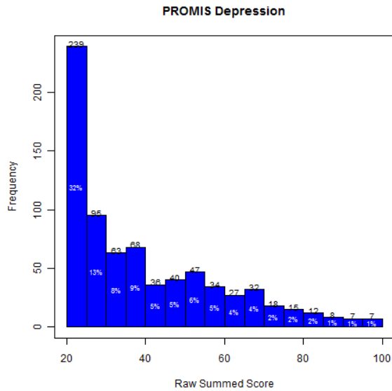
Figure 5.16.1: Raw Summed Score Distribution - PROMIS Instrument
