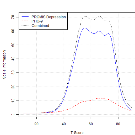
Figure 5.16.7: Comparison of Scale Information Functions
