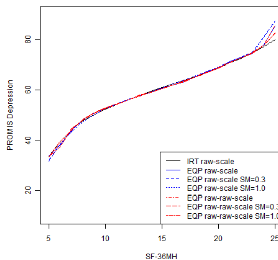
Figure 5.4.10: Equipercentile Linking Functions
