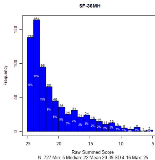
Figure 5.4.2: Raw Summed Score Distribution - Linking Instrument
