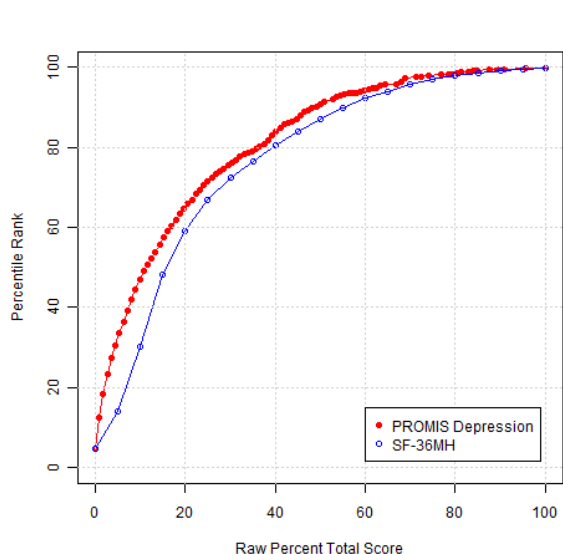
Figure 5.4.9: Comparison of Cumulative Distribution Functions based on Raw Summed Scores
